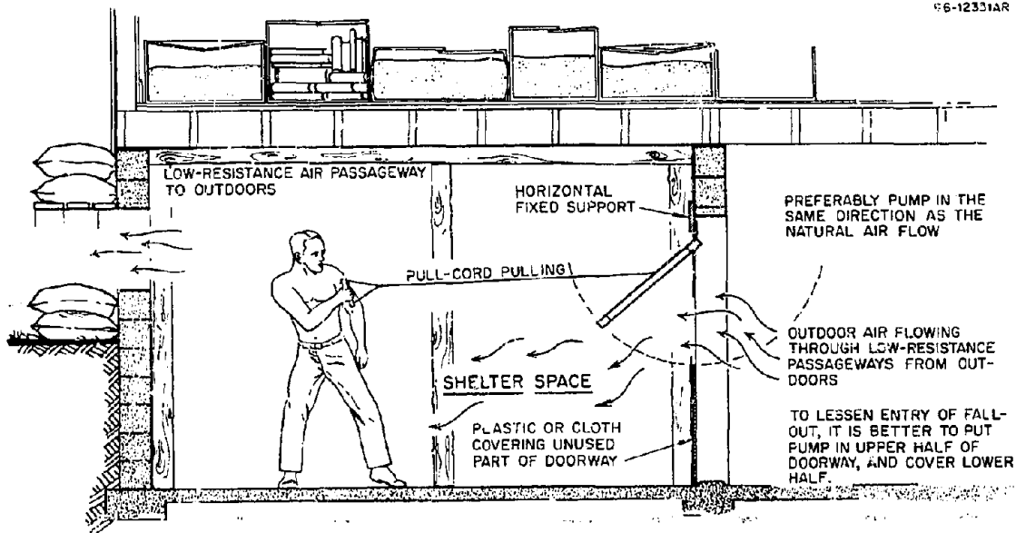
Fig. B-14. Installation of Kearny Air Pump.
